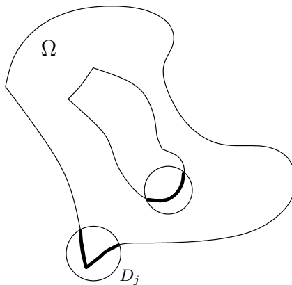
Figure 10. A domain with boundary Lipschitz arcs
