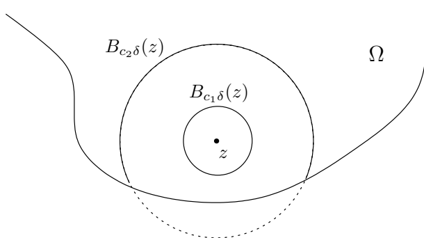
Figure 6. The situation in Proposition 4.13
