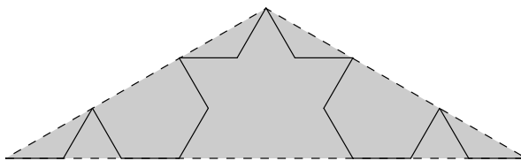
Figure 7. Open set in the separation of the von Koch similarities
